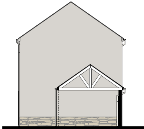
FACADE ARRIERE
